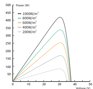
Power-Voltage Curve(420W)
