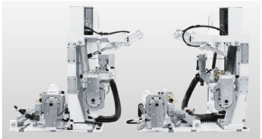
FF32 profile trimming unit For rounding edges on the front and rear edge of the workpiece at the top and bottom at different feed speeds.
