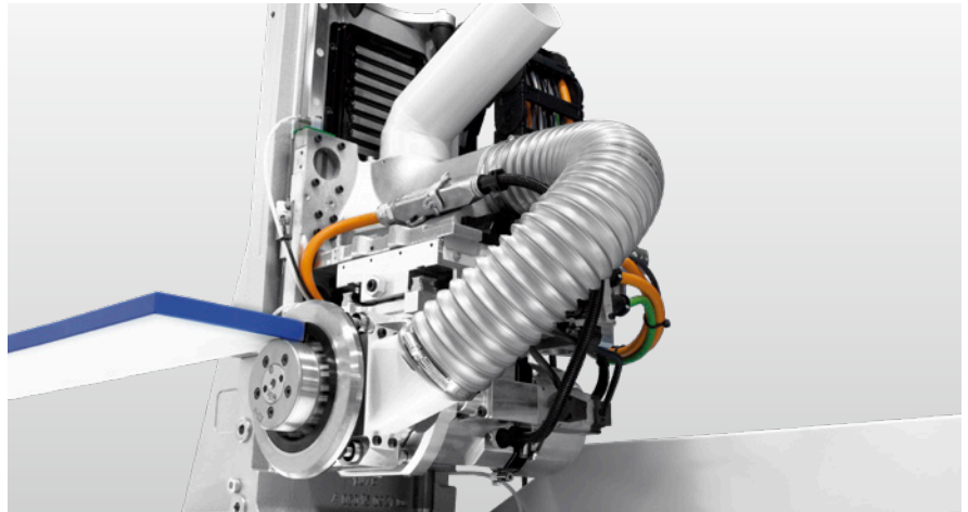
FK30 profile trimming unit For trimming around the front and rear edges.
